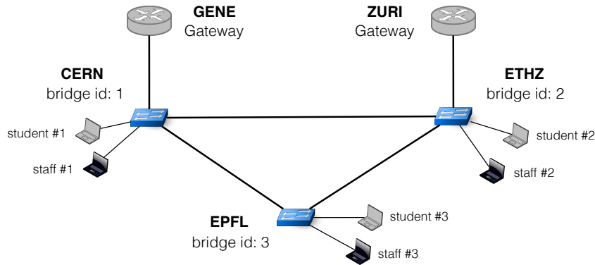
Figure 1: Layer-2 Topology
