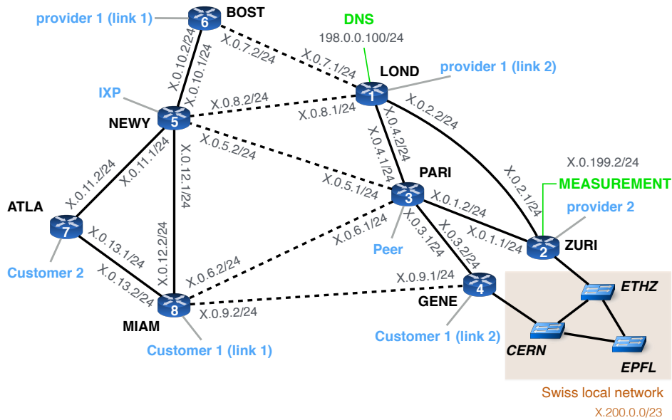
Figure 2: Layer-3 Topology
