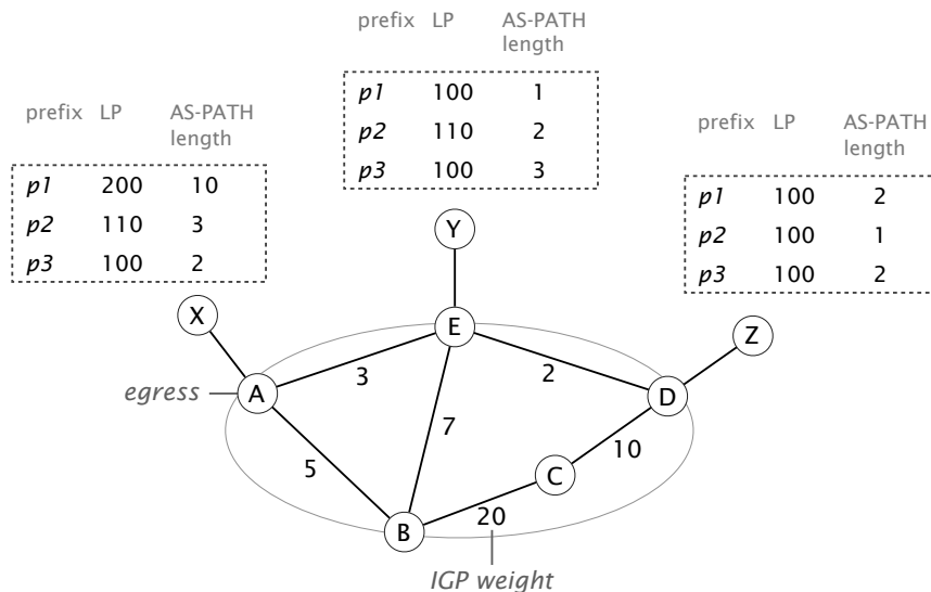
A simple ISP network which receives BGP routes for 3 different external prefixes ( p1, p2, p3 ) from 3 routers ( X, Y, Z ) located in neighboring ASes.
